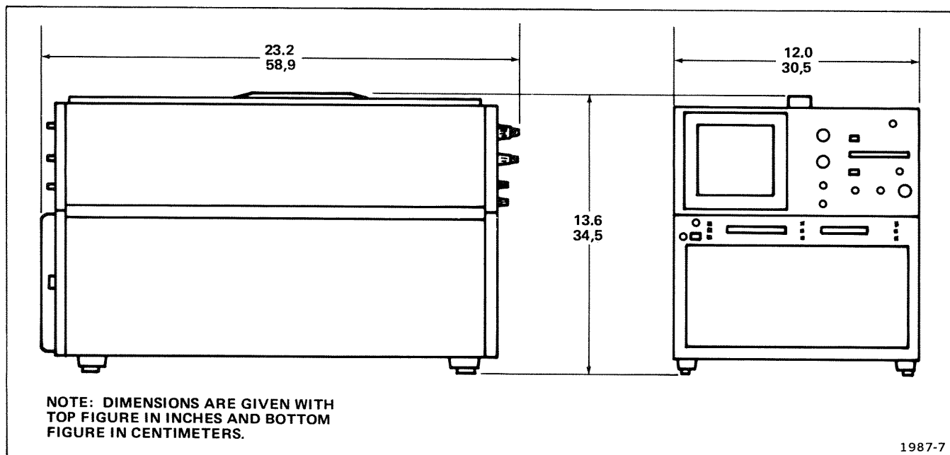
Figure 1-1. 7834 dimensional drawing.
